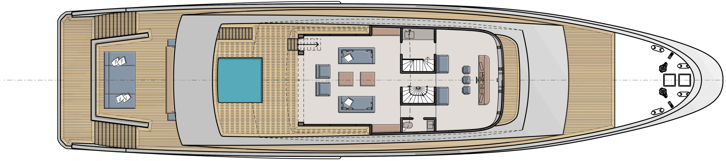
WHEELHOUSE DECK
