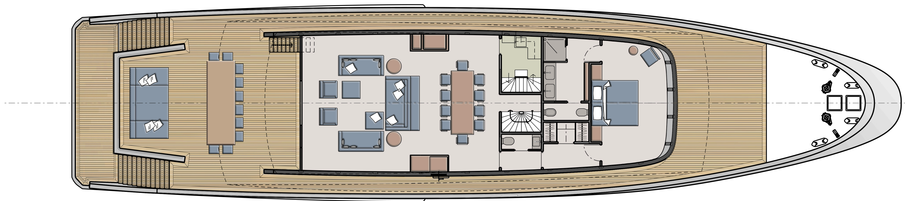
MAIN DECK
