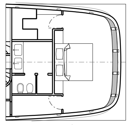
MAIN DECK
