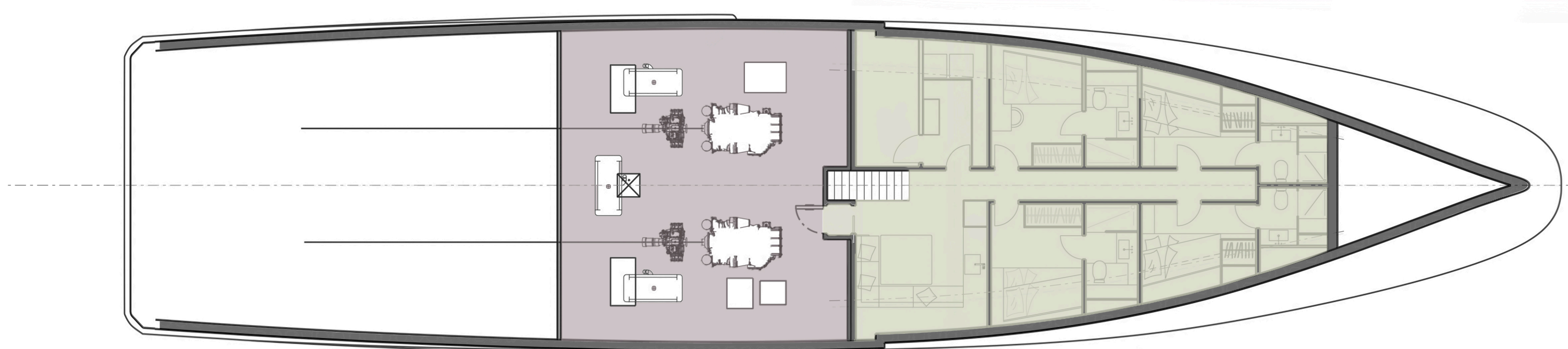
BOTTOM DECK
